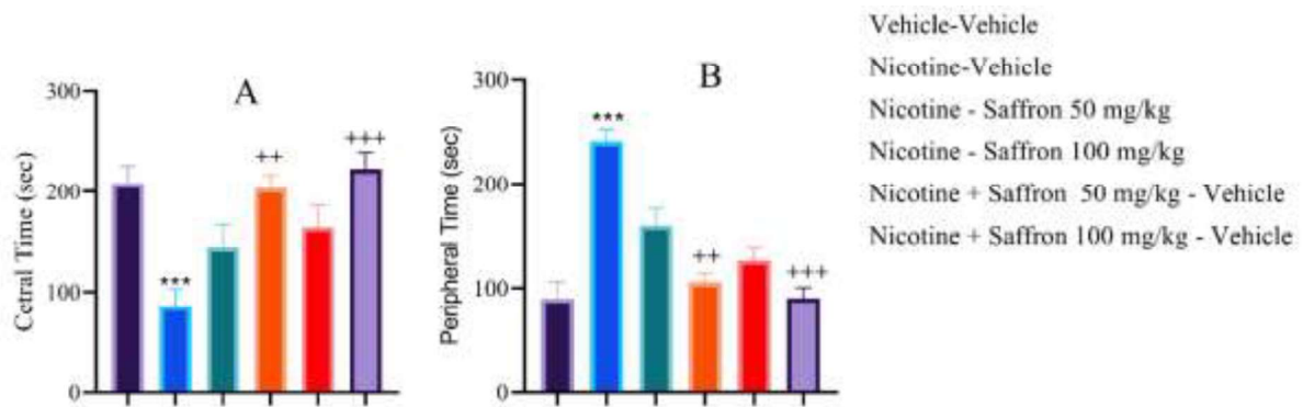
Fig. ۱: Effects of saffron on anxiety-like behaviors in the open field test (OFT). (A) Time spent in the central zone; (B) time spent in the peripheral zone across experimental groups. Data are expressed as mean \pm SEM. * p < ۰,۰۵ , *** p < ۰,۰۰۱ vs. vehicle-vehicle group; ++ p < ۰,۰۱ , +++ p < ۰,۰۰۱ vs. nicotine-vehicle group
