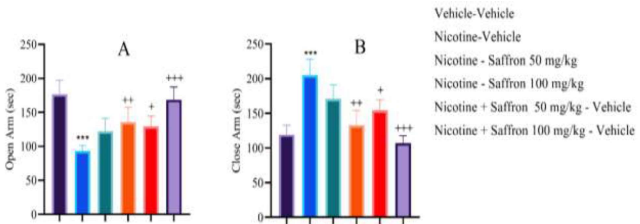
Fig. ۲: Effects of saffron on anxiety-like behaviors in the elevated plus maze (EPM). (A) Time spent in open arms; (B) time spent in enclosed arms across experimental groups. Data are expressed as mean \pm SEM. *** P < ۰,۰۰۱ vs. vehicle-vehicle group; + P < ۰,۰۵ , ++ P < ۰,۰۱ , +++ P < ۰,۰۰۱ vs. nicotine-vehicle group
