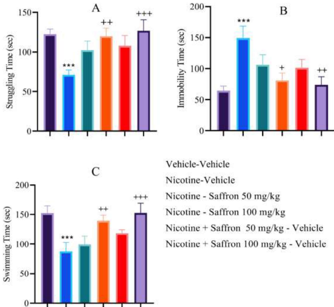
Fig. ۳: Effects of saffron on depressive-like behaviors in the forced swim test (FST). (A) Time spent struggling; (B) immobility duration; (C) swimming time across experimental groups. Data are expressed as mean \pm SEM. *** P < 0.001 vs. vehicle-vehicle group; + P < 0.05 , ++ P < 0.01 , +++ P < 0.001 vs. nicotine-vehicle group
